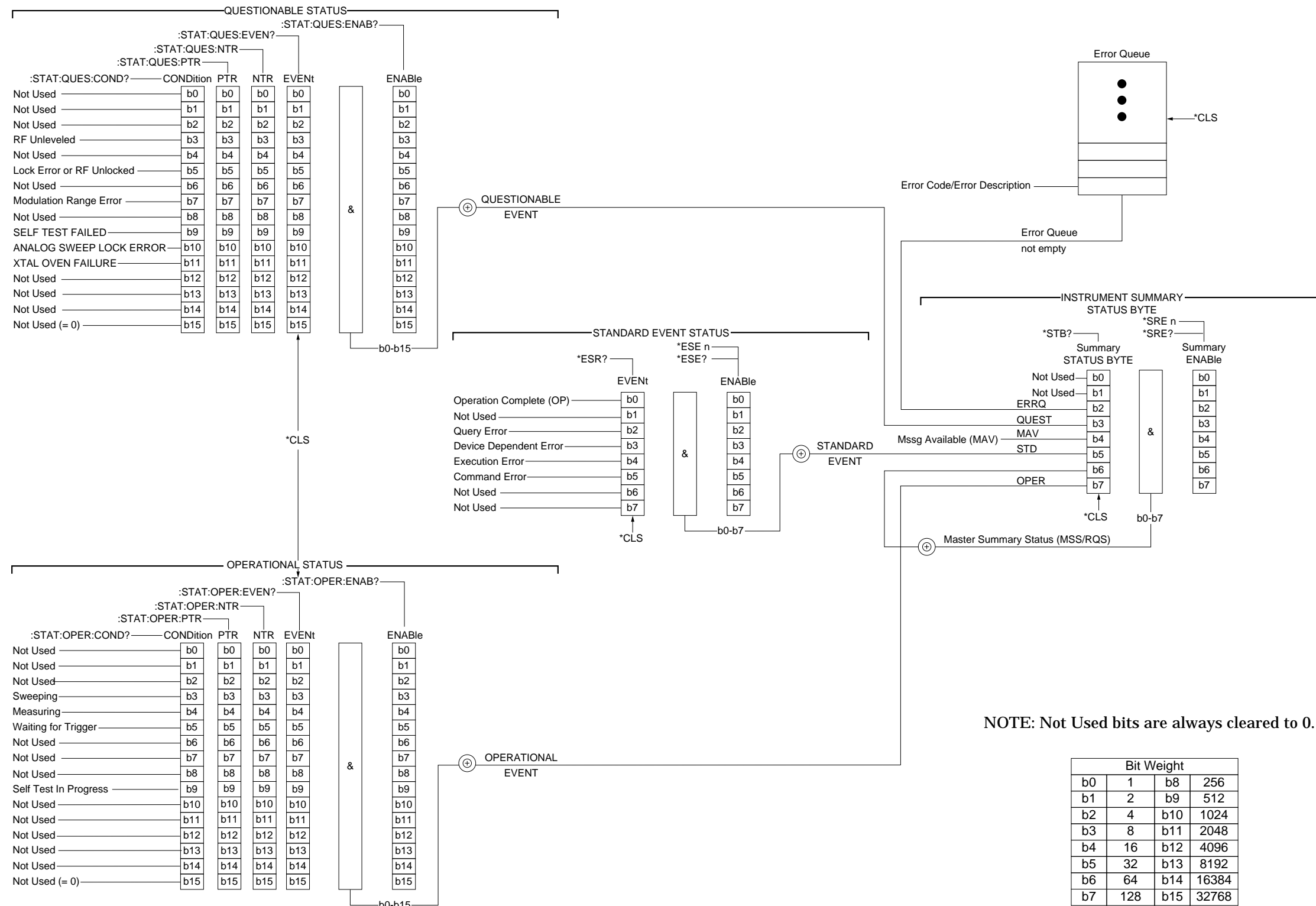
Figure 2-1. 692XXA/693XXA Status-Reporting Structure
